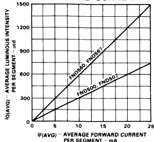
AVERAGE LUMINOUS INTENSITY VERSUS AVERAGE FORWARD CURRENT
