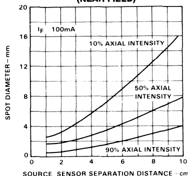
SPOT DIAMETER VERSUS SEPARATION DISTANCE (NEAR FIELD)
