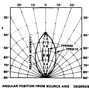
RADIATION PATTERN
