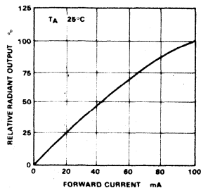
RADIANT OUTPUT VERSUS DC FORWARD CURRENT
