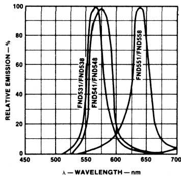
EMISSION SPECTRUM
