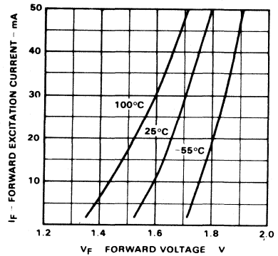
FORWARD CURRENT VERSUS FORWARD VOLTAGE
