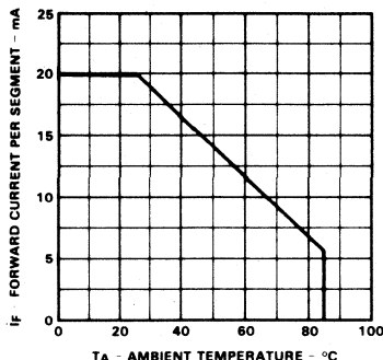
MAXIMUM AVERAGE CURRENT RATING VERSUS AMBIENT TEMPERATURE
