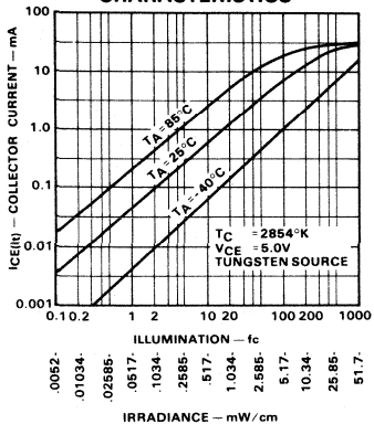
PHOTO CURRENT CHARACTERISTICS
