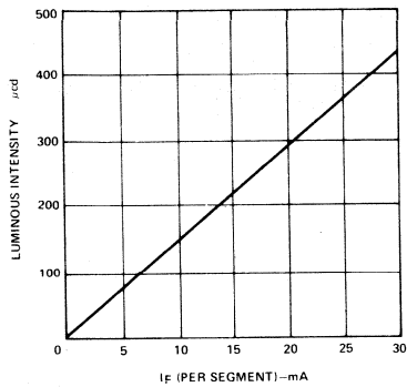
LUMINOUS INTENSITY VERSUS FORWARD CURRENT
