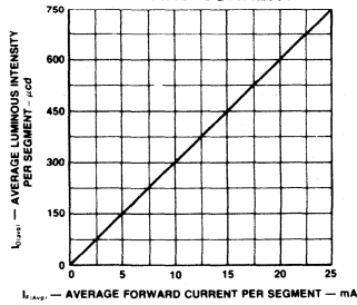
AVERAGE LUMINOUS INTENSITY VERSUS AVERAGE FORWARD CURRENT
