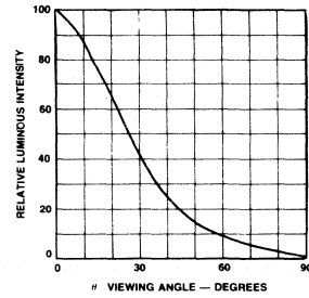
ANGULAR DISTRIBUTION OF LUMINOUS INTENSITY
