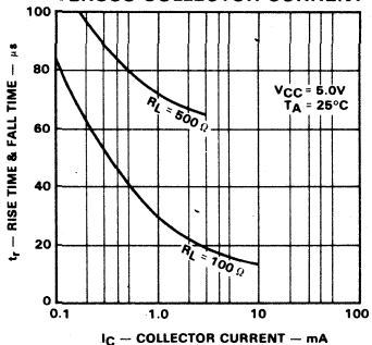
RISE AND FALL TIME VERSUS COLLECTOR CURRENT
