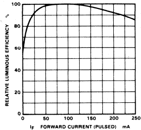
RELATIVE LUMINOUS EFFICIENCY (mcd PER mA) VERSUS PEAK CURRENT PER SEGMENT
