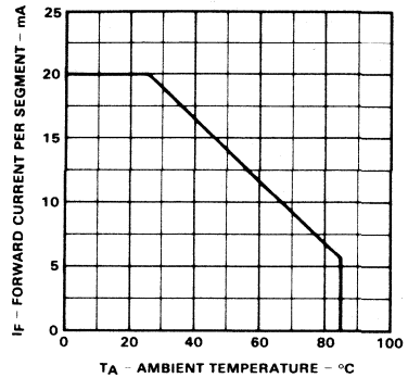
MAXIMUM AVERAGE CURRENT RATING VERSUS AMBIENT TEMPERATURE
