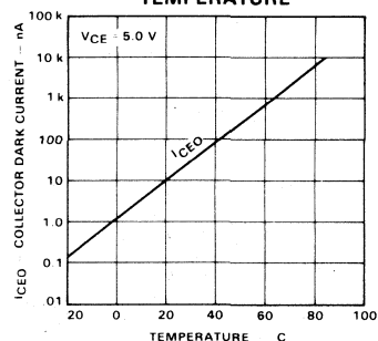
COLLECTOR DARK CURRENT VERSUS TEMPERATURE
