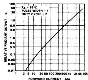
RADIANT OUTPUT VERSUS FORWARD CURRENT (PULSED)
