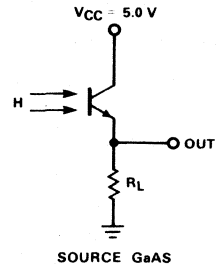
SWITCHING CIRCUIT FOR RISE AND FALL TIMES
