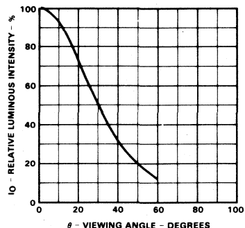
ANGULAR DISTRIBUTION OF LUMINOUS INTENSITY
