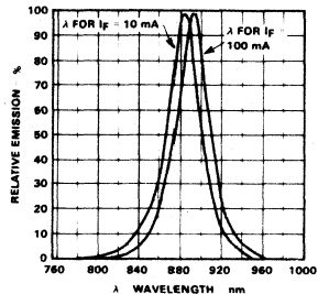
TYPICAL EMISSION SPECTRUM
