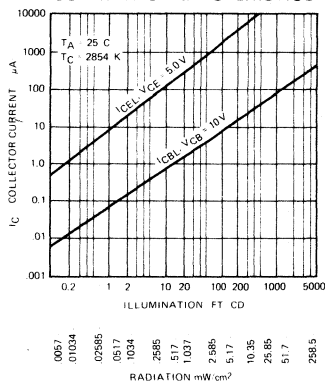
FPT100/A/B PHOTO CURRENT CHARACTERISTICS
