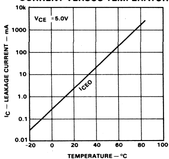
COLLECTOR DARK CURRENT VERSUS TEMPERATURE
