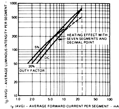
AVERAGE LUMINOUS INTENSITY VERSUS AVERAGE FORWARD CURRENT
