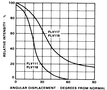
INTENSITY VERSUS VIEWING ANGLE
