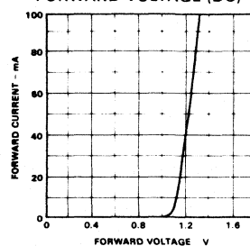
FORWARD CURRENT VERSUS FORWARD VOLTAGE (DC)
