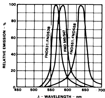
EMISSION SPECTRUM
