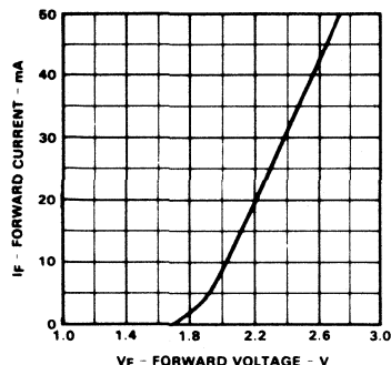
FORWARD CURRENT VERSUS FORWARD VOLTAGE
