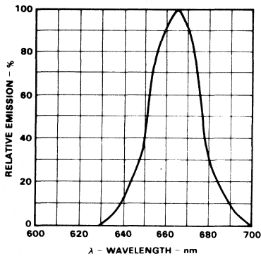
EMISSION SPECTRUM
