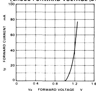
FORWARD CURRENT VERSUS FORWARD VOLTAGE (D.C.)
