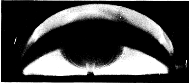
CZOCHEKRALSKI CRYSTAL GROWER
