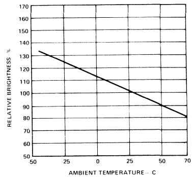
LUMINOUS INTENSITY VERSUS TEMPERATURE
