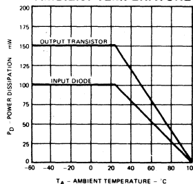
MAXIMUM POWER DISSIPATION RATING VERSUS AMBIENT TEMPERATURE
