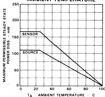
MAXIMUM P_D VERSUS AMBIENT TEMPERATURE
