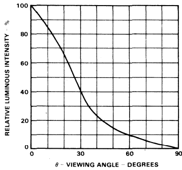
ANGULAR DISTRIBUTION OF LUMINOUS INTENSITY
