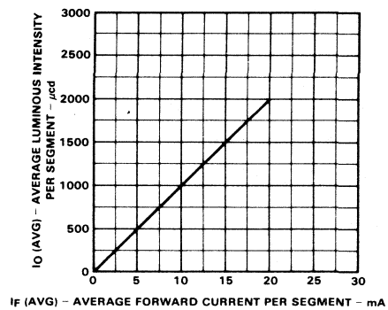
AVERAGE LUMINOUS INTENSITY VERSUS AVERAGE FORWARD CURRENT
