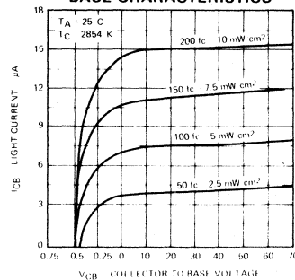
COLLECTOR BASE CHARACTERISTICS
