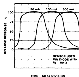
RADIANT EMISSION TRANSIENT RESPONSE
