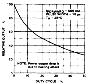
RADIANT OUTPUT VERSUS DUTY CYCLE
