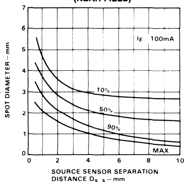
SPOT DIAMETER VERSUS SEPARATION DISTANCE (NEAR FIELD)
