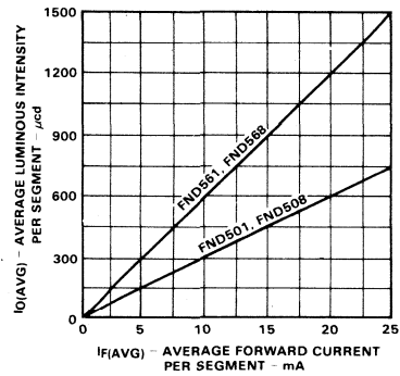
AVERAGE LUMINOUS INTENSITY VERSUS AVERAGE FORWARD CURRENT
