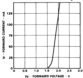
FORWARD CURRENT VERSUS FORWARD VOLTAGE ( T_J )
