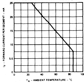
MAXIMUM AVERAGE CURRENT RATING VERSUS AMBIENT TEMPERATURE
