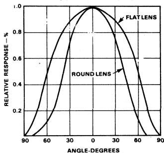
ANGULAR RESPONSE
