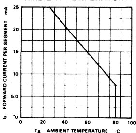
MAXIMUM AVERAGE CURRENT RATING VERSUS AMBIENT TEMPERATURE
