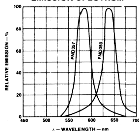
EMISSION SPECTRUM
